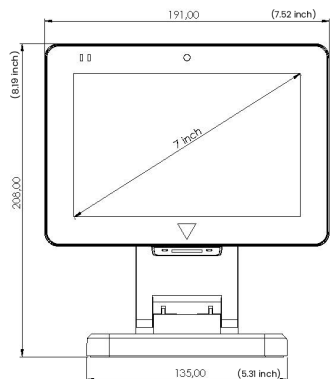
Desk stand
